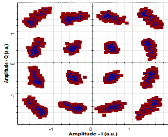
Fig. 8: Constellation diagram of 16-QAM
