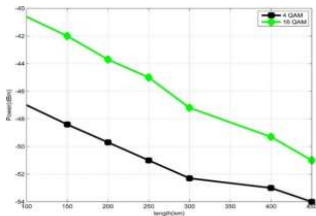
Fig. 5: Power versus the length of optical fiber.
