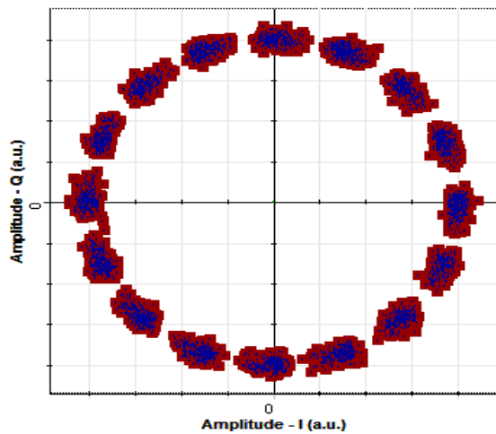
Fig. 7: Constellation diagram of 16-DPSK.
