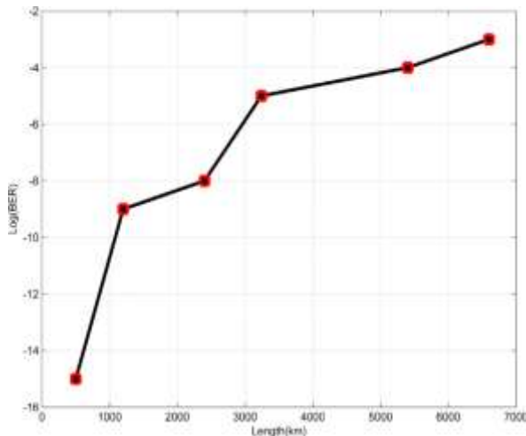
Fig.9: BER vs. transmission distance for 1.65Tbps data rate.
